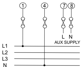
1 Phase 2 Wire
